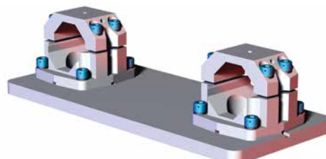
60mm Double Extrusion Robot Adaptor Mid Mount (Blank Plate)
