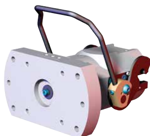
Style 23 - MD350 (Ø187mm Bolt Circle)
