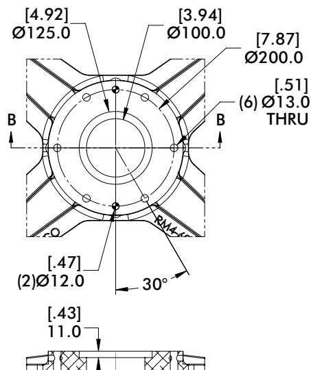
R17 (Ø160mm Bolt Circle)
