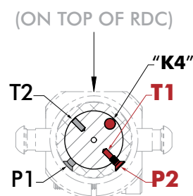
"K4" POSITION FASTENER IN (P2/T1)
