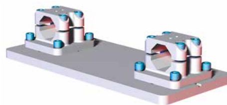
45mm Double Extrusion Robot Adaptor Mid Mount (Blank Plate)
