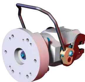
Style 21 - EOAMC30 (Ø127mm Bolt Circle/ Ø108mm Dowel Circle)
